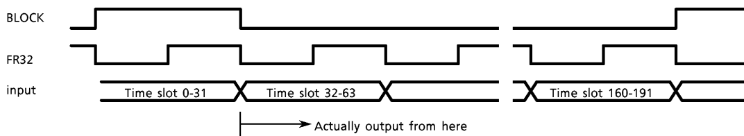
Figure 6 192 Bit Input Timing Example
